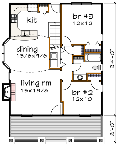
Floor 1 plan
