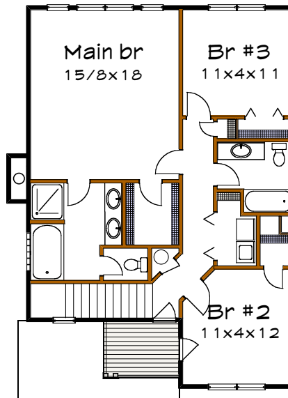
Floor 2 plan
